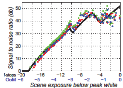
Figure 2b: Simulated vs. measured PSNR
