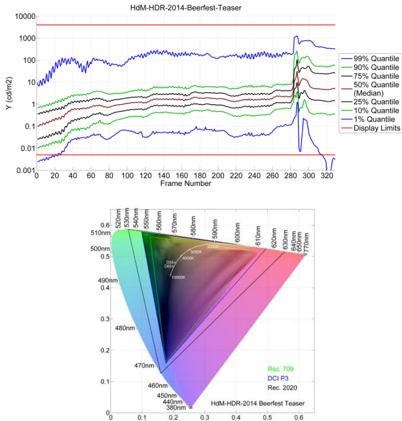
Figure 3: Beerfest Teaser Percentiles and CIE1976 u'v' Chromaticity Diagram
