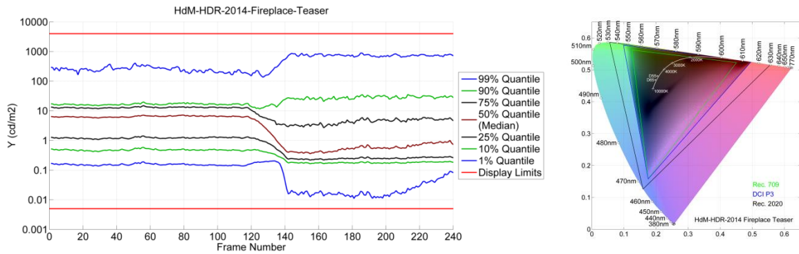
Figure 4: Fireplace Teaser snapshot(#76), Percentiles and CIE1976 u'v' Chromaticity Diagram
